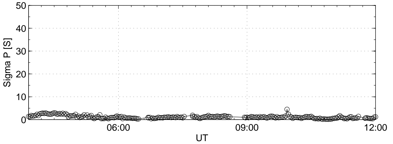
2001-01-22 tau0@42m Sigma P
