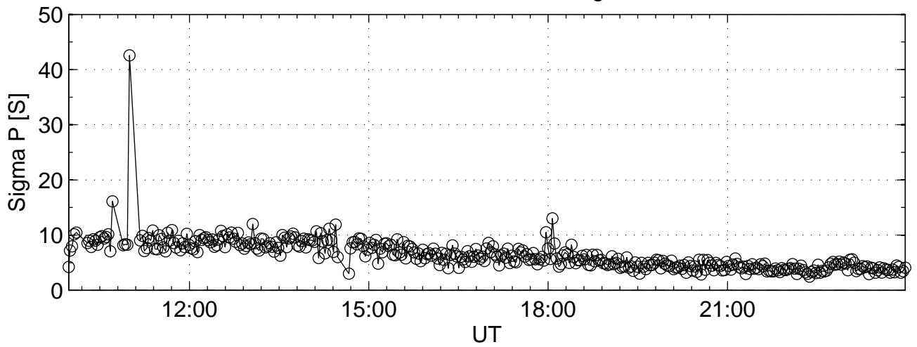
2001-07-11 tau0@42m Sigma P
