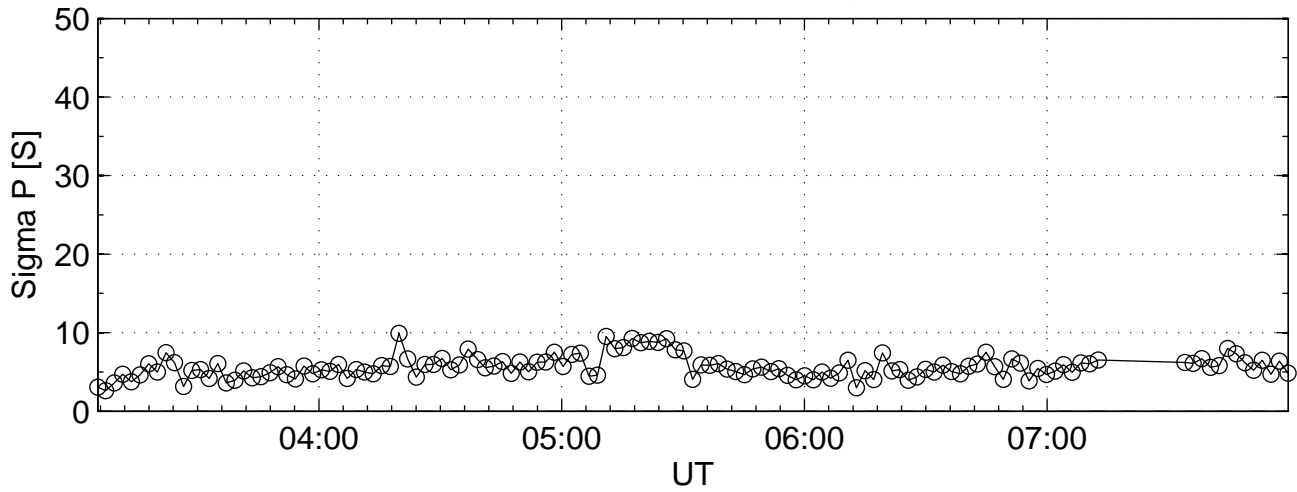
2002-08-01 tau0@42m Sigma P
