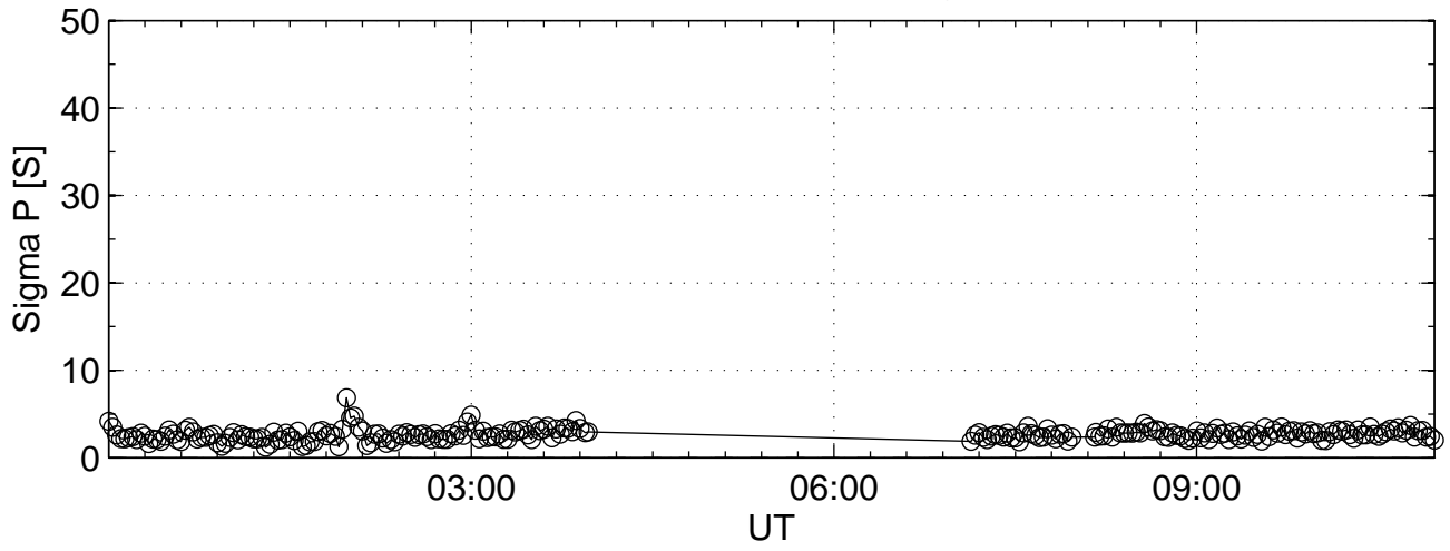
2002-08-26 tau0@42m Sigma P
