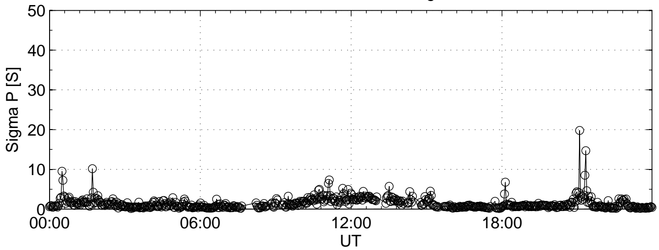
2002-10-30 tau0@42m Sigma P
