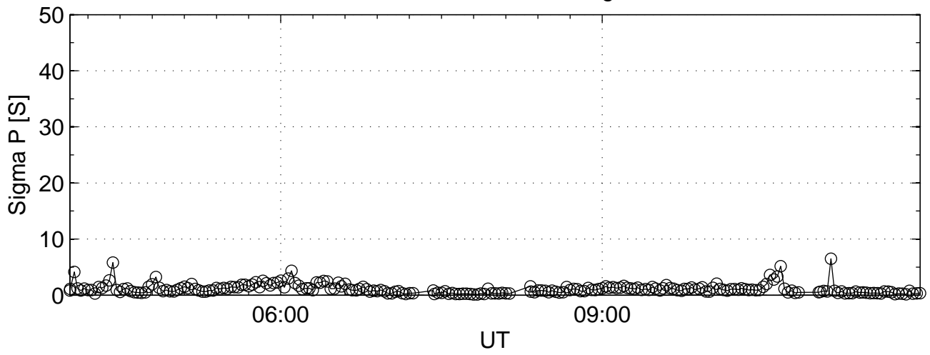
2004-01-21 tau0@42m Sigma P
