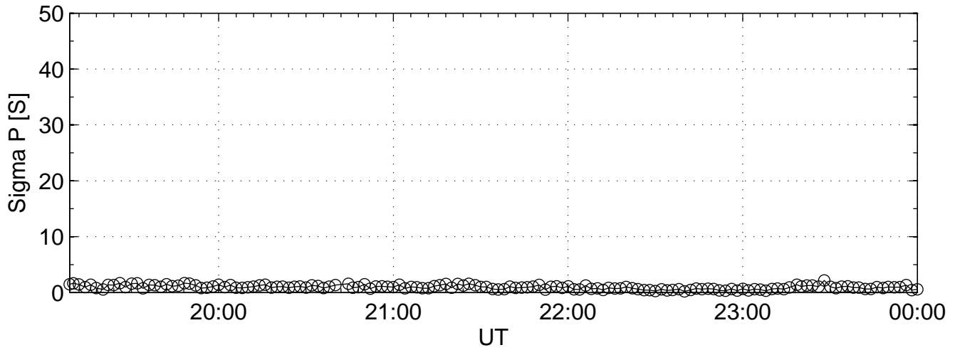
2004-09-02 tau0@42m Sigma P
