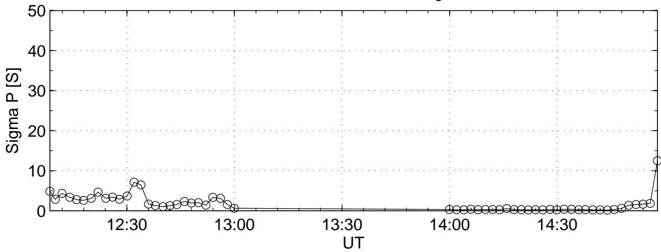
2004-12-11 steffe@42m Sigma P
