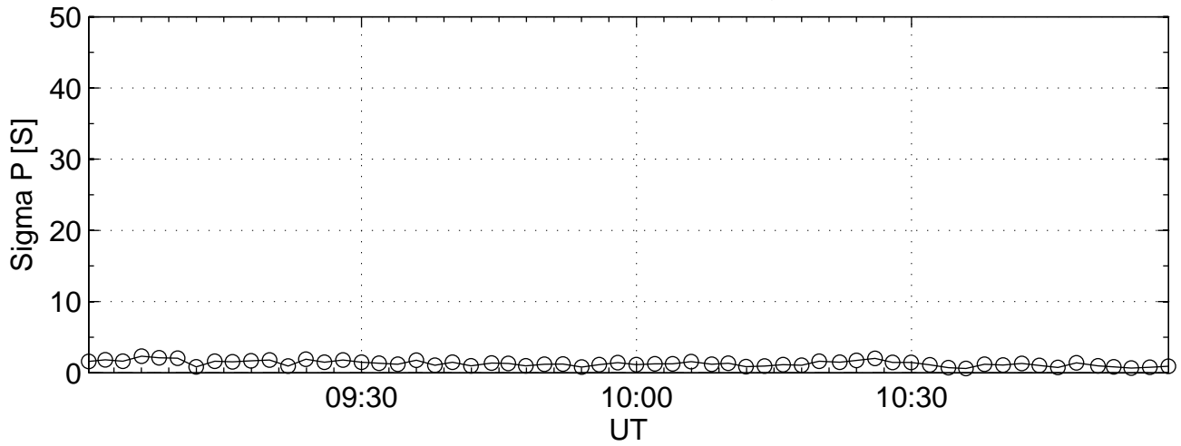
2005-01-31 tau0@42m Sigma P
