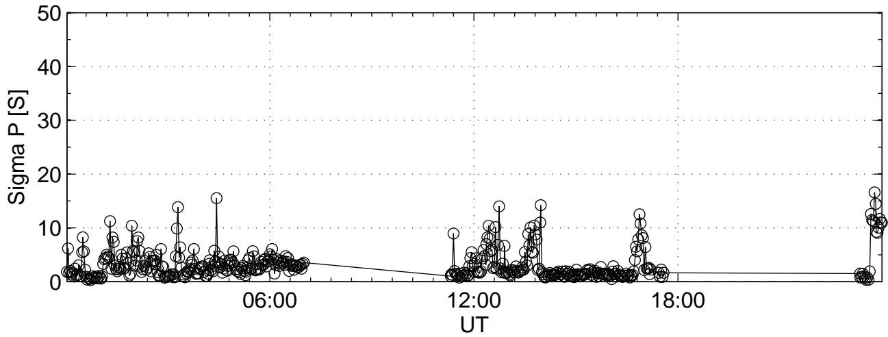
2006-12-14 tau0@42m Sigma P
