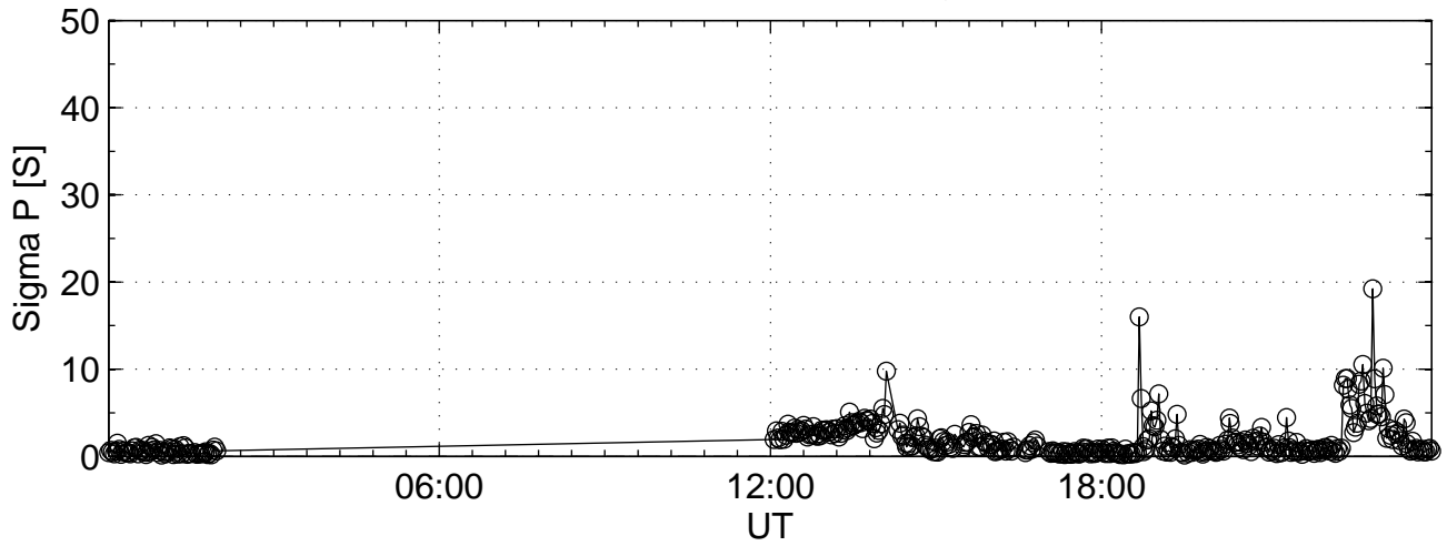
2006-12-18 tau0@42m Sigma P
