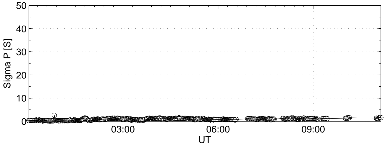
2007-10-11 ipy@42m Sigma P
