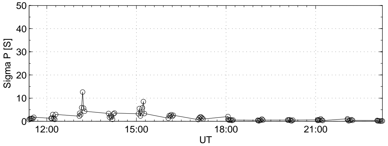
2007-12-04 tau0@42m Sigma P
