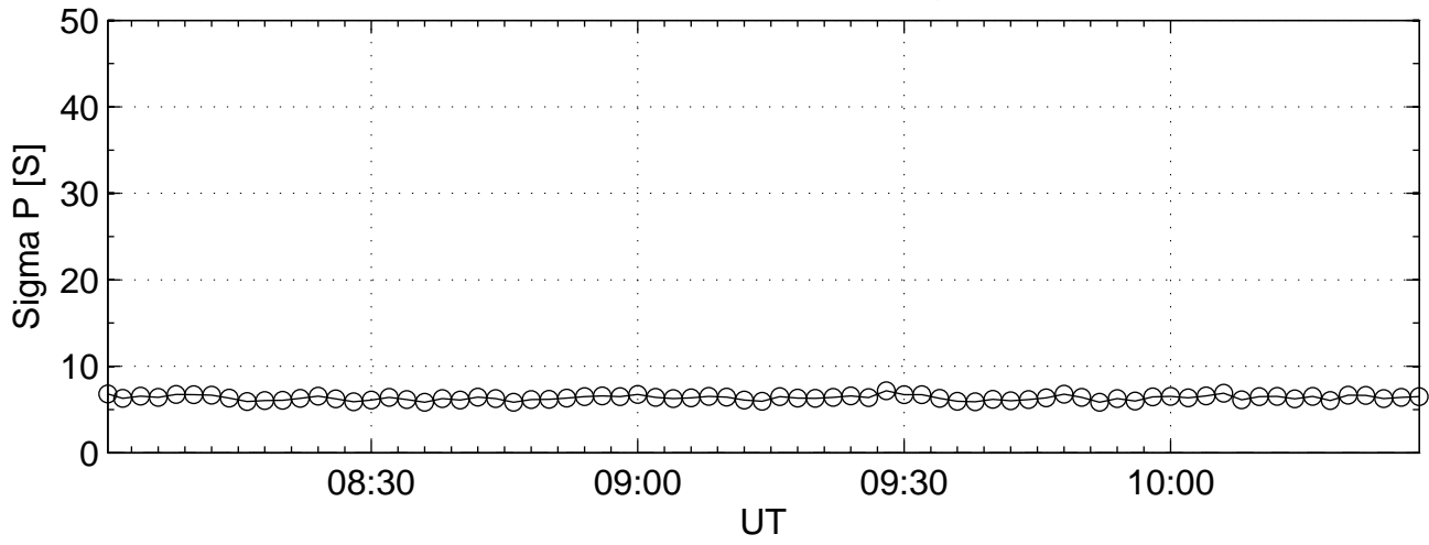
2009-08-18 tau7@42m Sigma P
