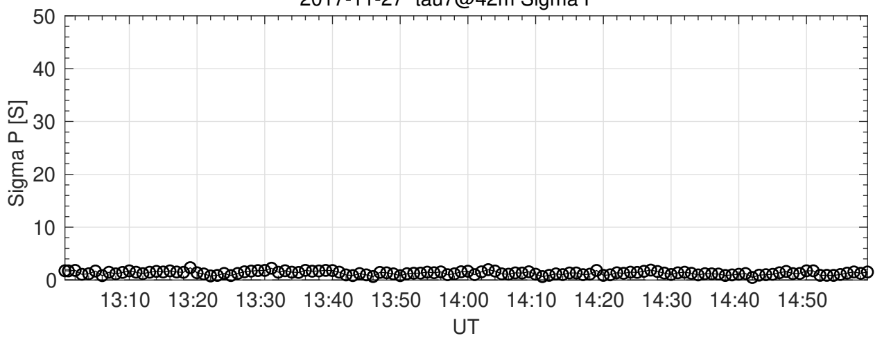
2017-11-27 tau7@42m Sigma P
