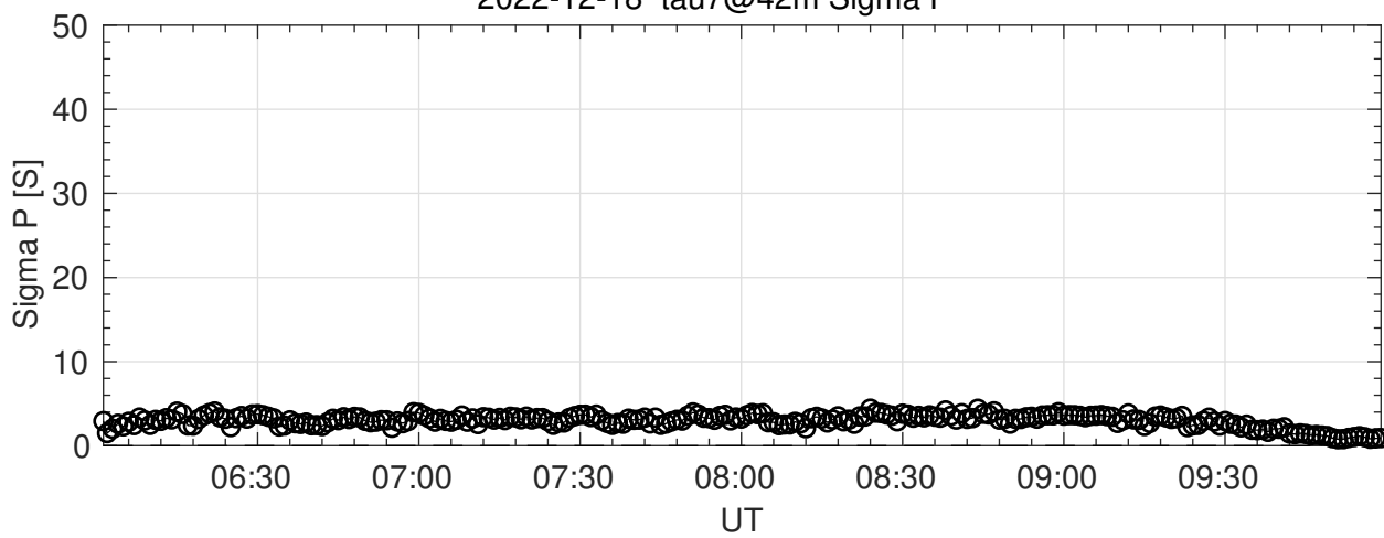
2022-12-18 tau7@42m Sigma P
