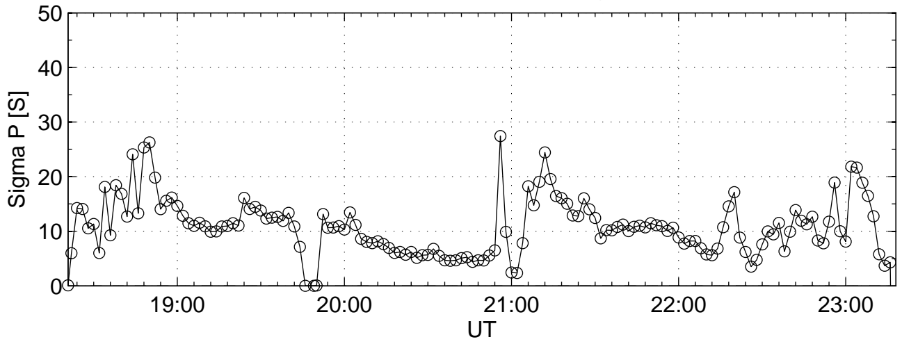
1995-01-30 PULSE@uhf Sigma P
