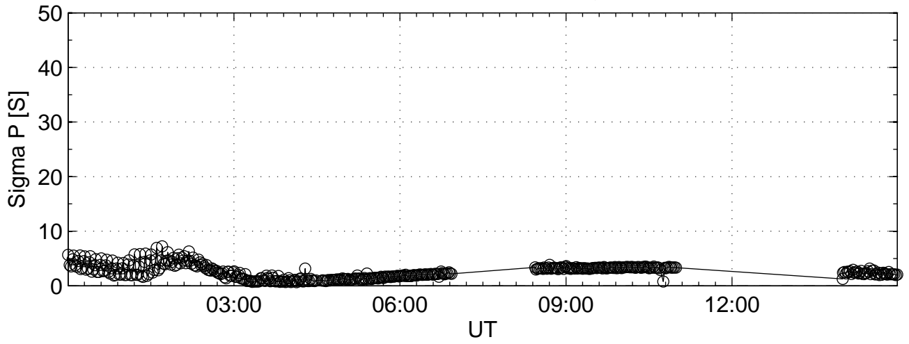
2005-09-29 tau2pl@uhf Sigma P
