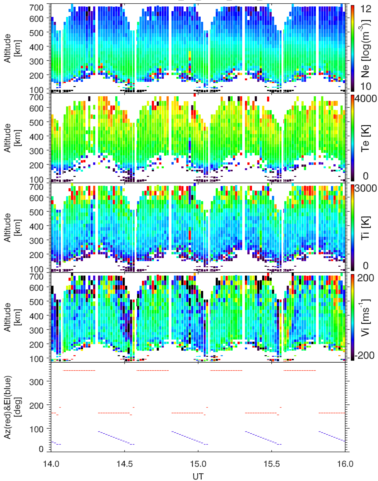
EISCAT 1998-04-27_14_16UT_gup0_ant@32m.
