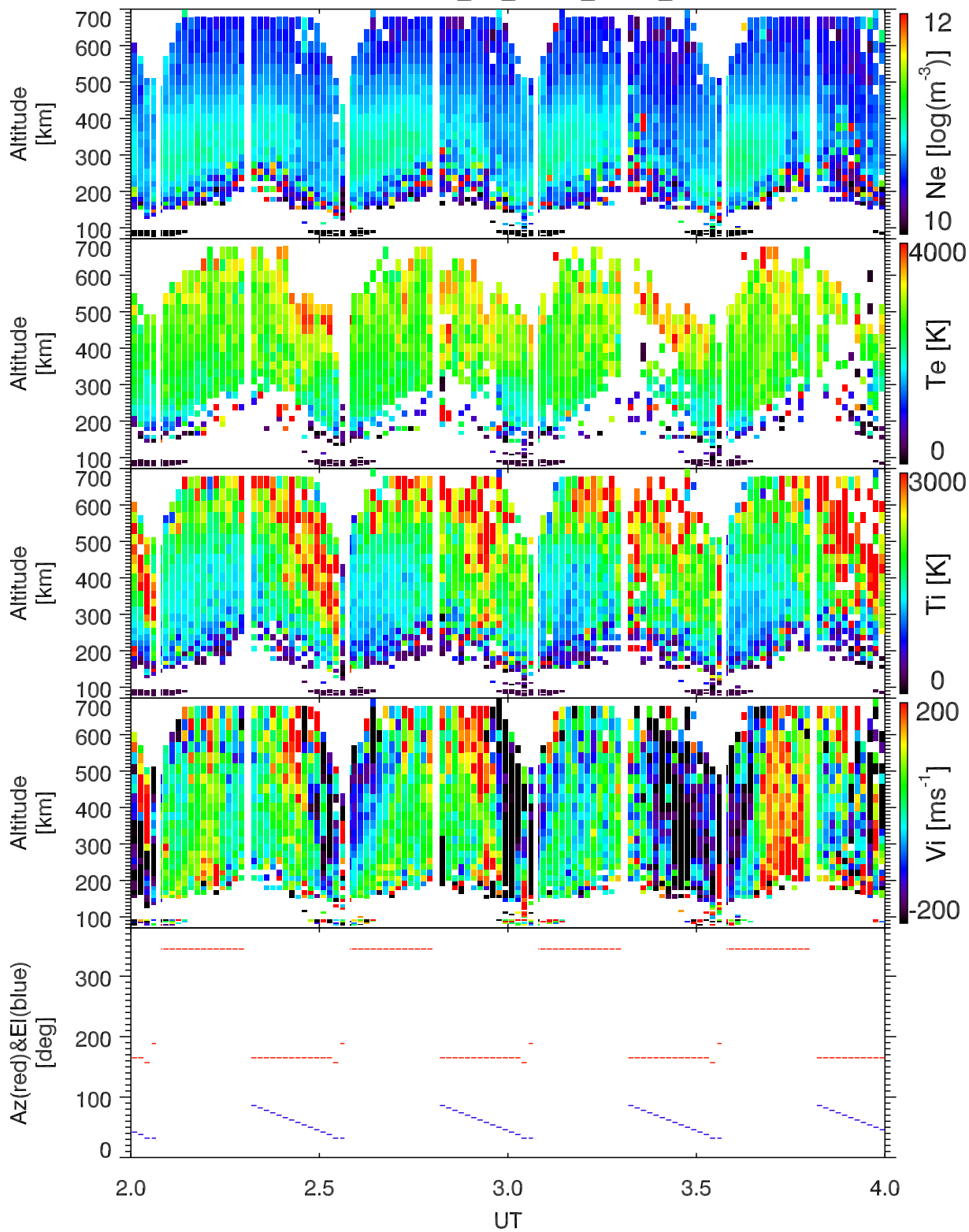
EISCAT 1998-04-28_02_04UT_gup0_ant@32m.
