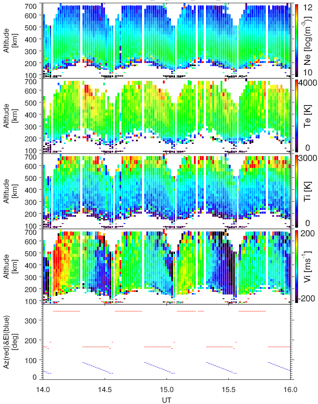
EISCAT 1998-04-28_14_16UT_gup0_ant@32m.
