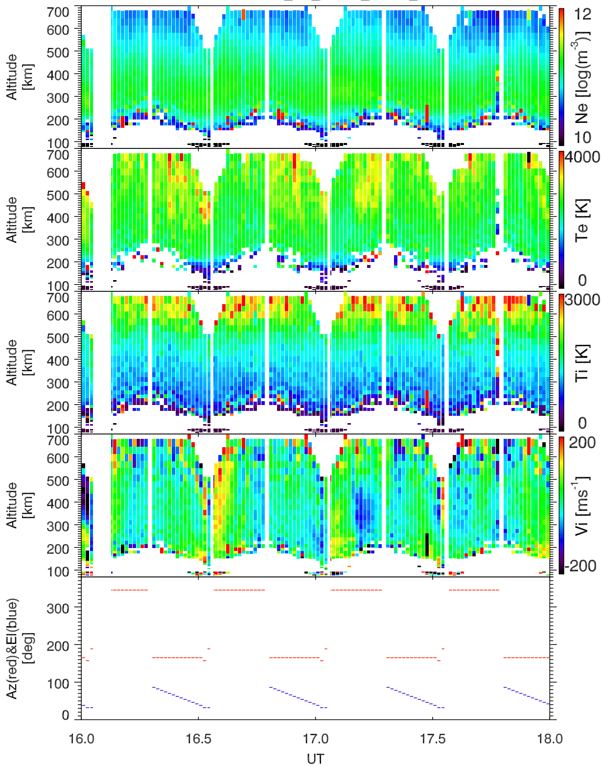
EISCAT 1998-04-30_16_18UT_gup0_ant@32m.
