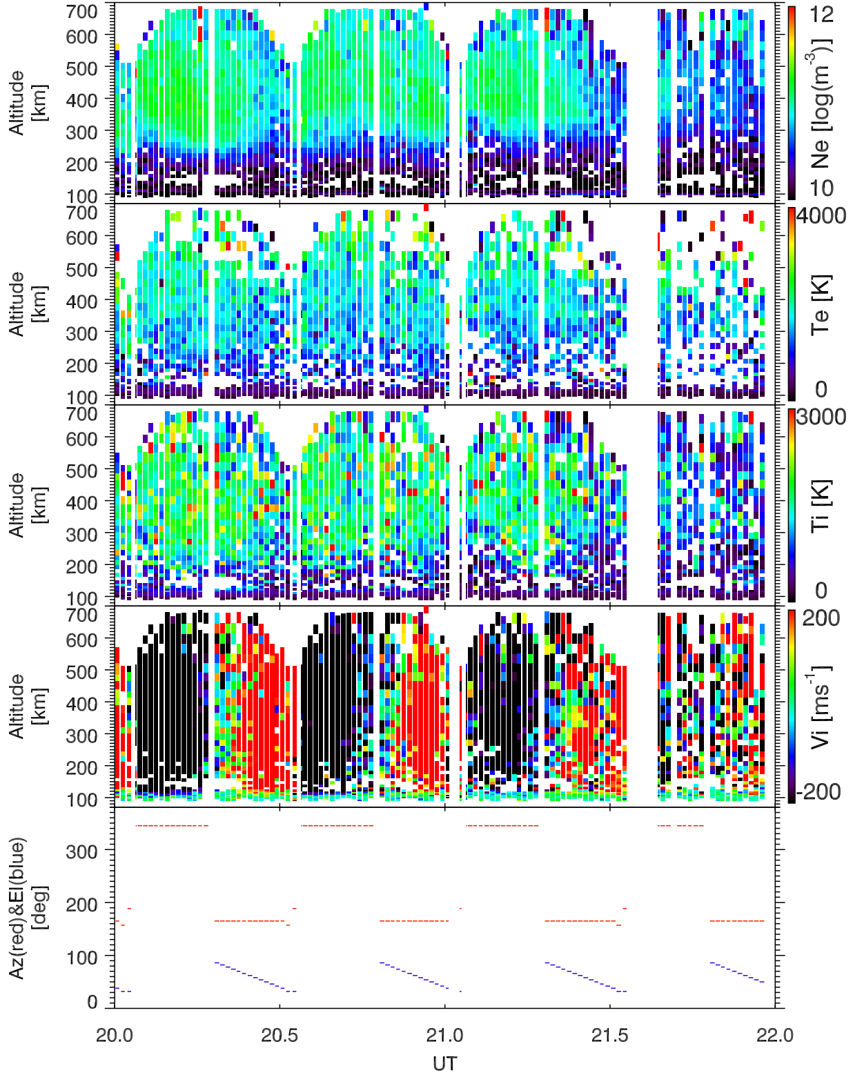
EISCAT 1998-10-19_20_22UT_gup3c_ant@32m.
