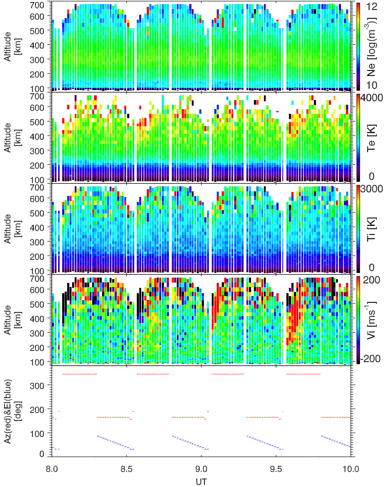
EISCAT 1999-04-22_08_10UT_gup3c_ant@32m.
