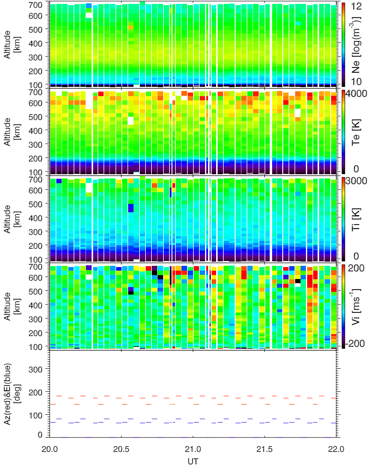
EISCAT 1999-07-03_20_22UT_gup3c_ant@32m.
