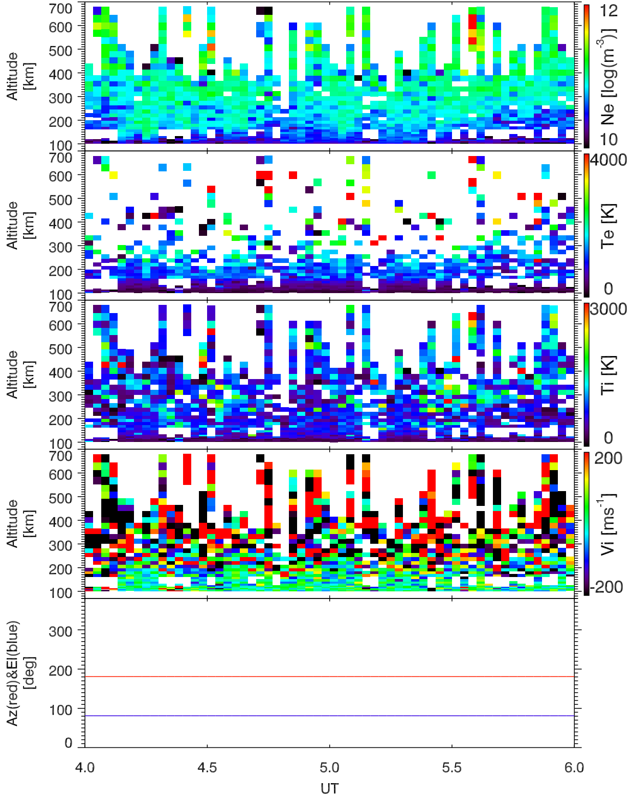
EISCAT 2000-01-07_04_06UT_gup3c_120@42m.
