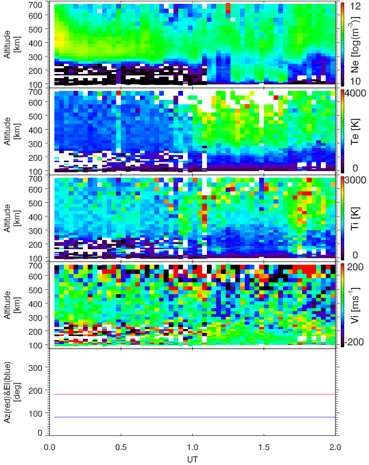
EISCAT 2000-02-10_00_02UT_gup3c_120@42m.
