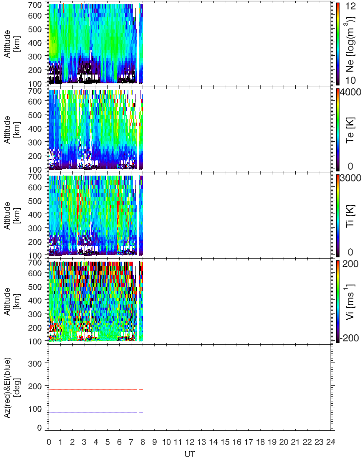
EISCAT 2000-02-10_00_24UT_gup3c_120@42m.
