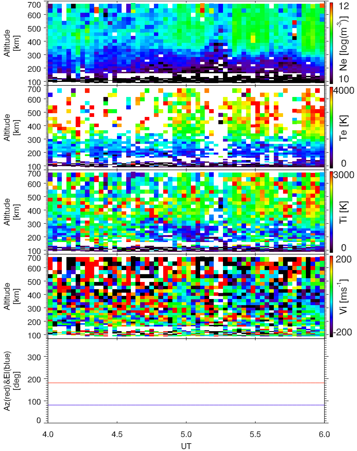
EISCAT 2000-02-24_04_06UT_gup3c_120@42m.
