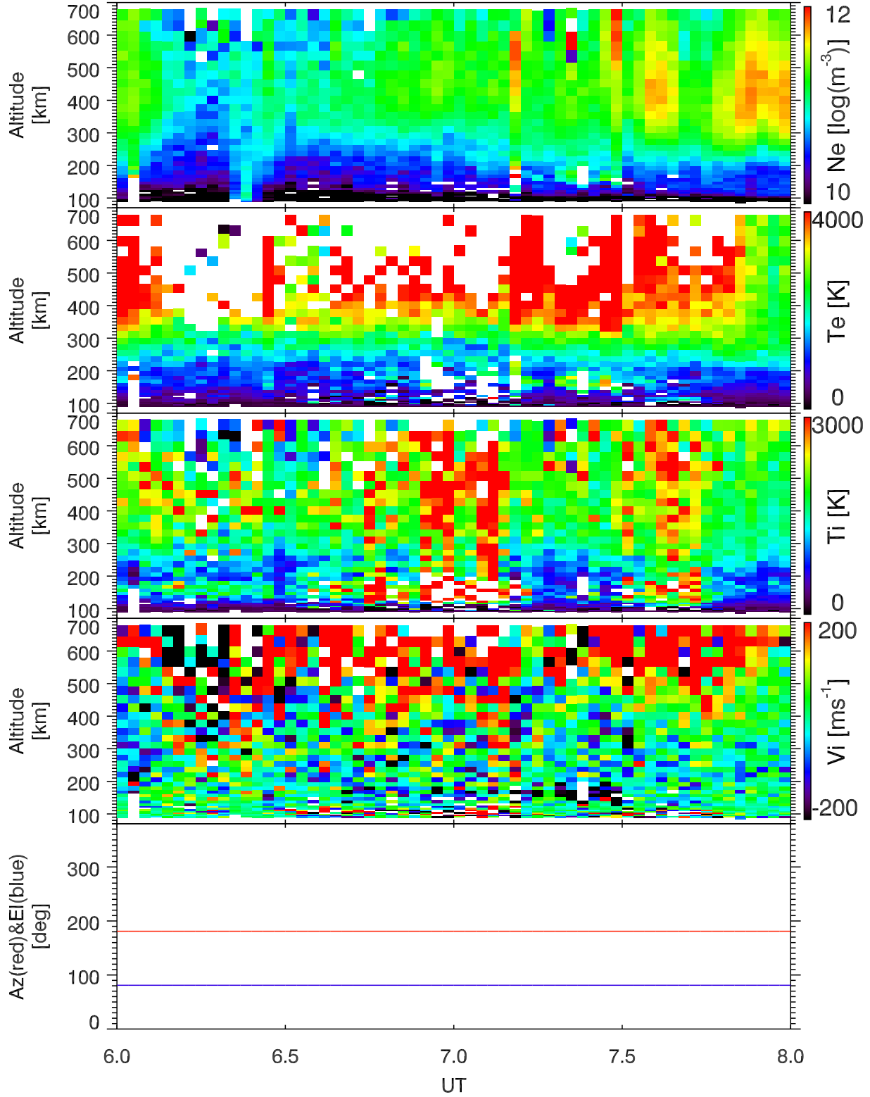
EISCAT 2000-02-24_06_08UT_gup3c_120@42m.
