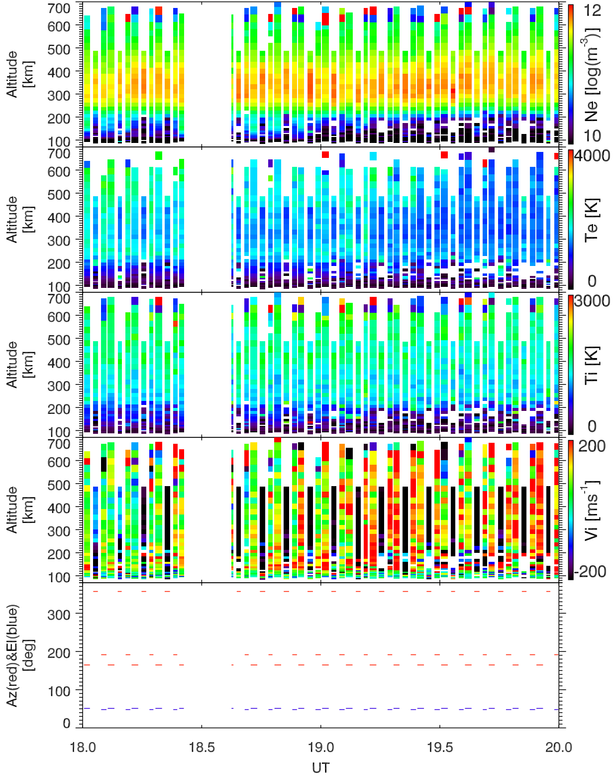
EISCAT 2000-03-14_18_20UT_gup3c_ant@32m.
