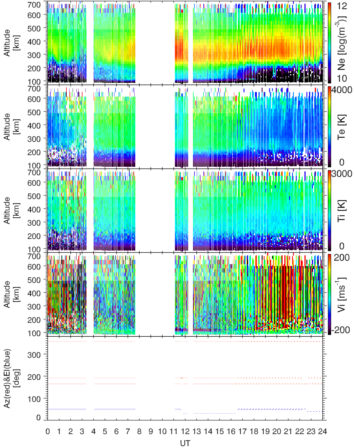
EISCAT 2000-03-15_00_24UT_gup3c_ant@32m.
