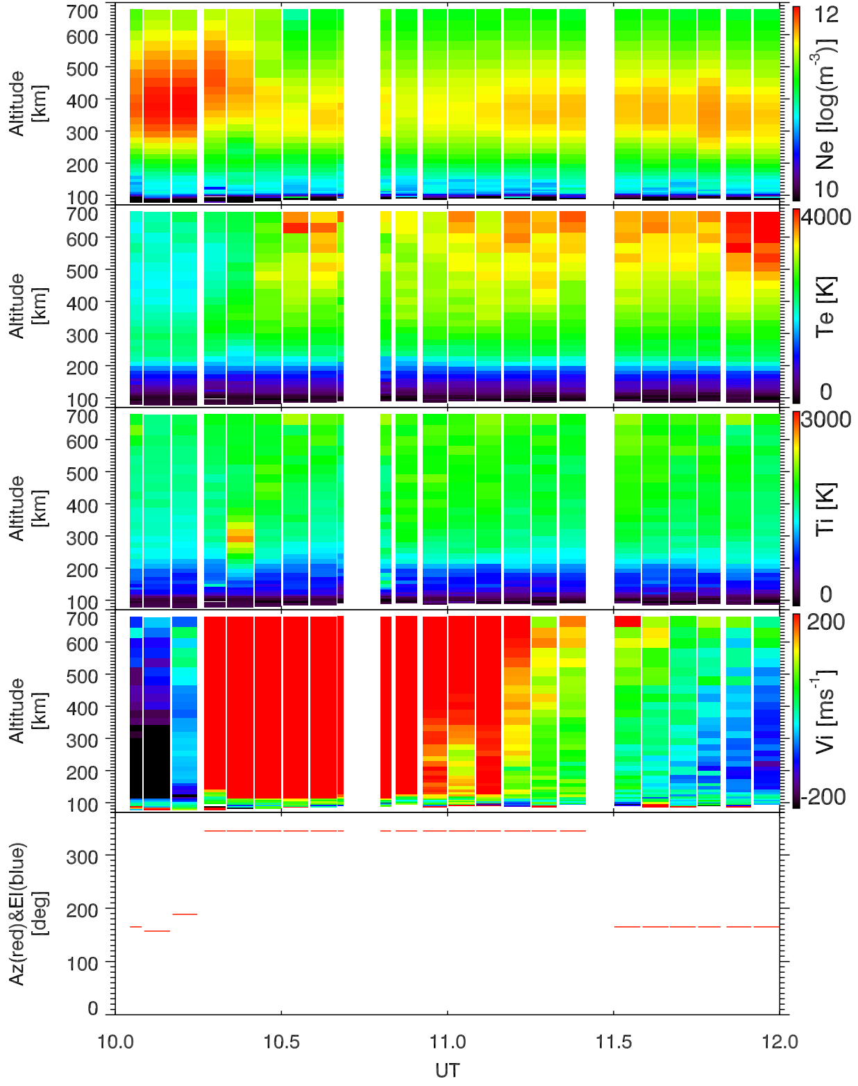
EISCAT 2000-04-11_10_12UT_tau0_ant@32m.
