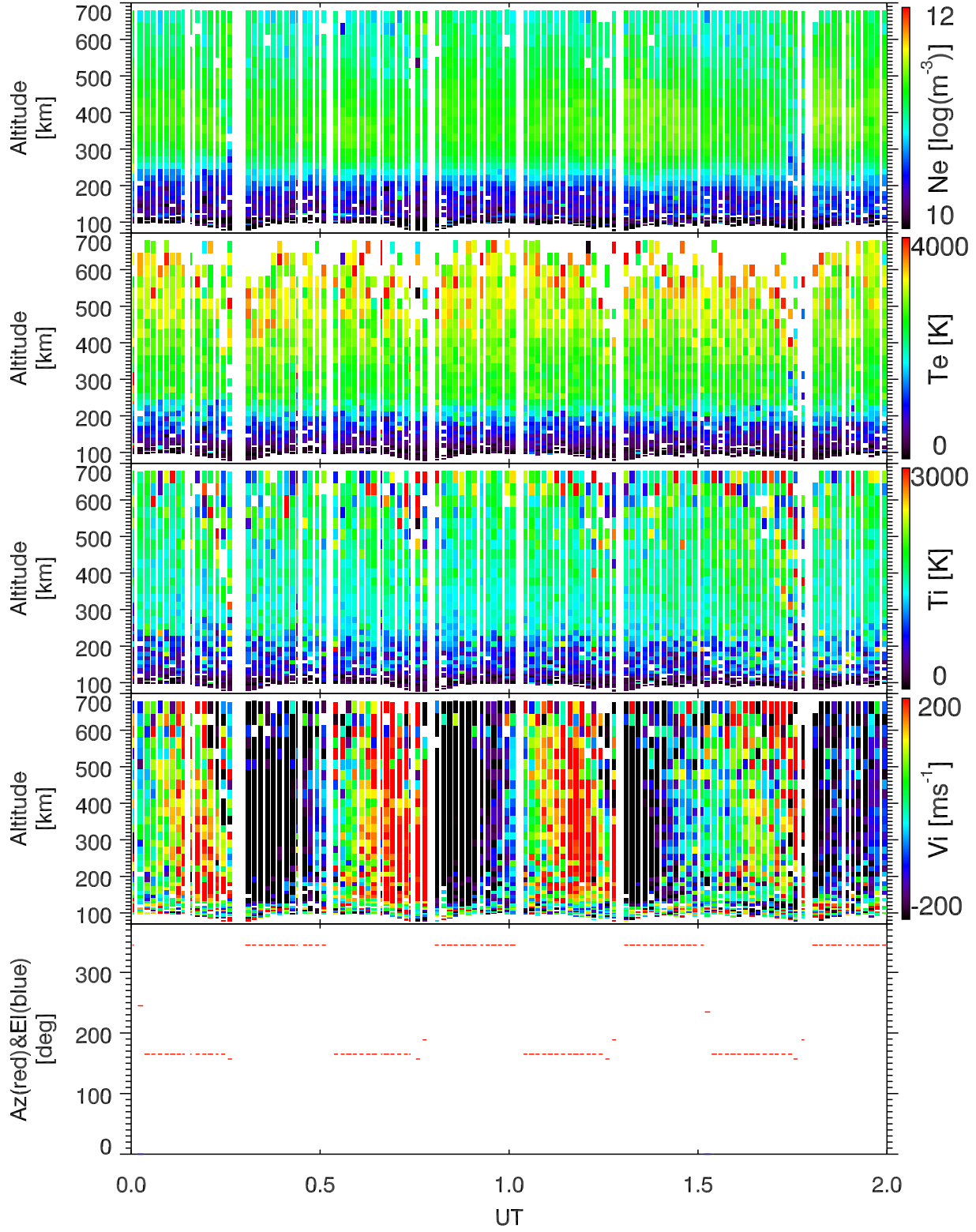
EISCAT 2000-04-12_00_02UT_tau0_ant@32m.
