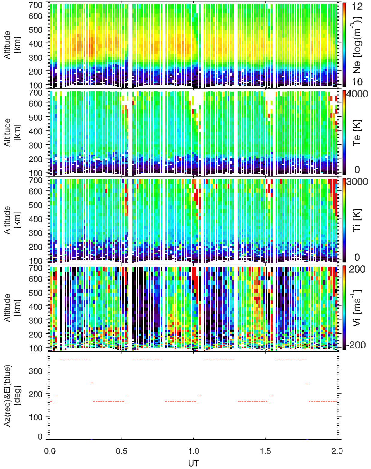
EISCAT 2000-04-13_00_02UT_tau0_ant@32m.
