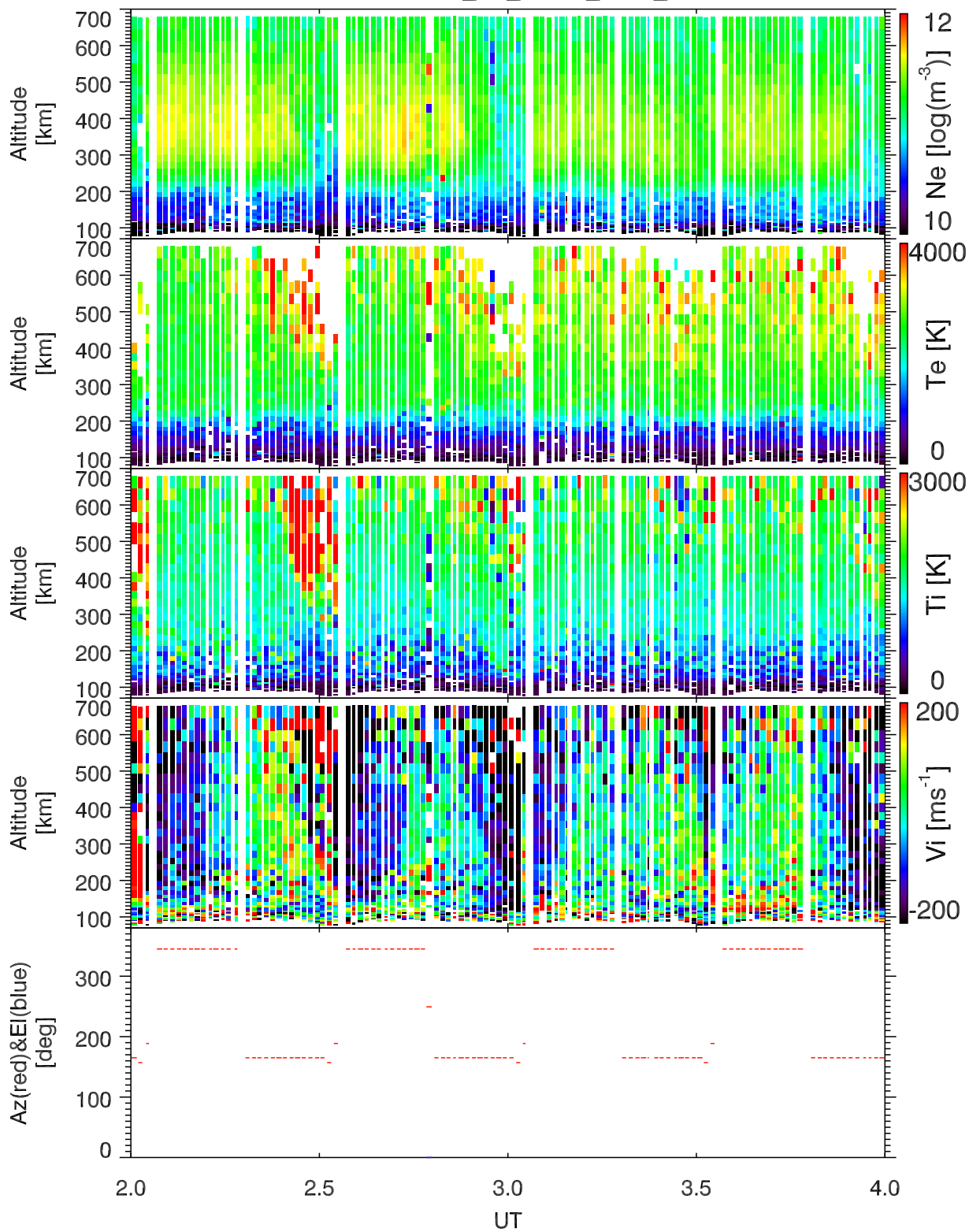
EISCAT 2000-04-13_02_04UT_tau0_ant@32m.
