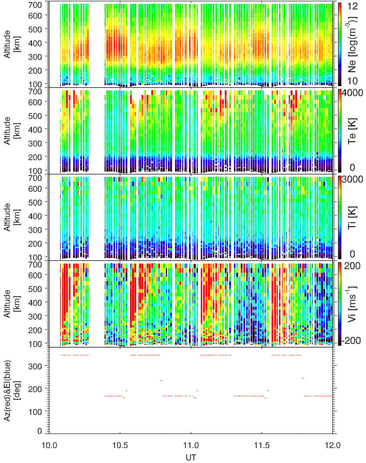
EISCAT 2000-04-13_10_12UT_tau0_ant@32m.
