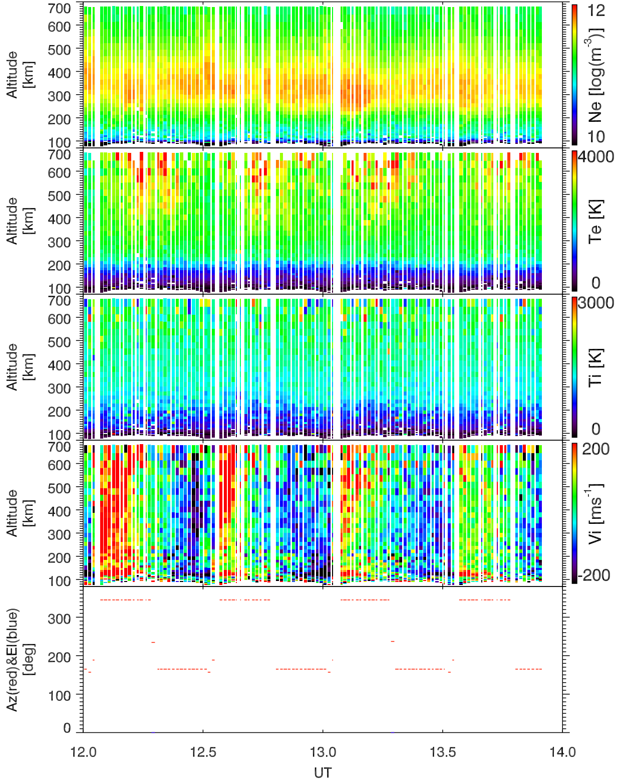
EISCAT 2000-04-13_12_14UT_tau0_ant@32m.
