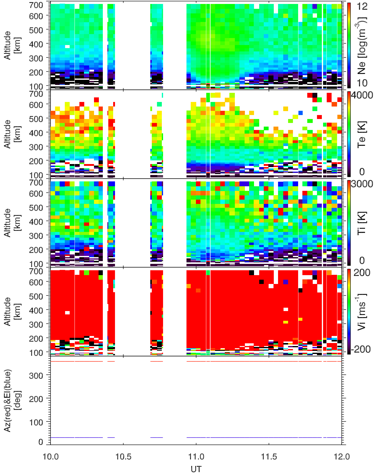
EISCAT 2000-07-15_10_12UT_tau0_120@32m.
