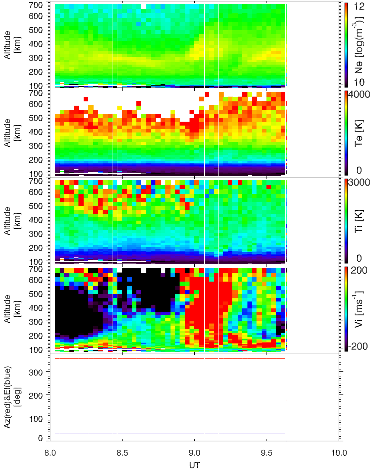
EISCAT 2000-07-17_08_10UT_tau0_120@32m.
