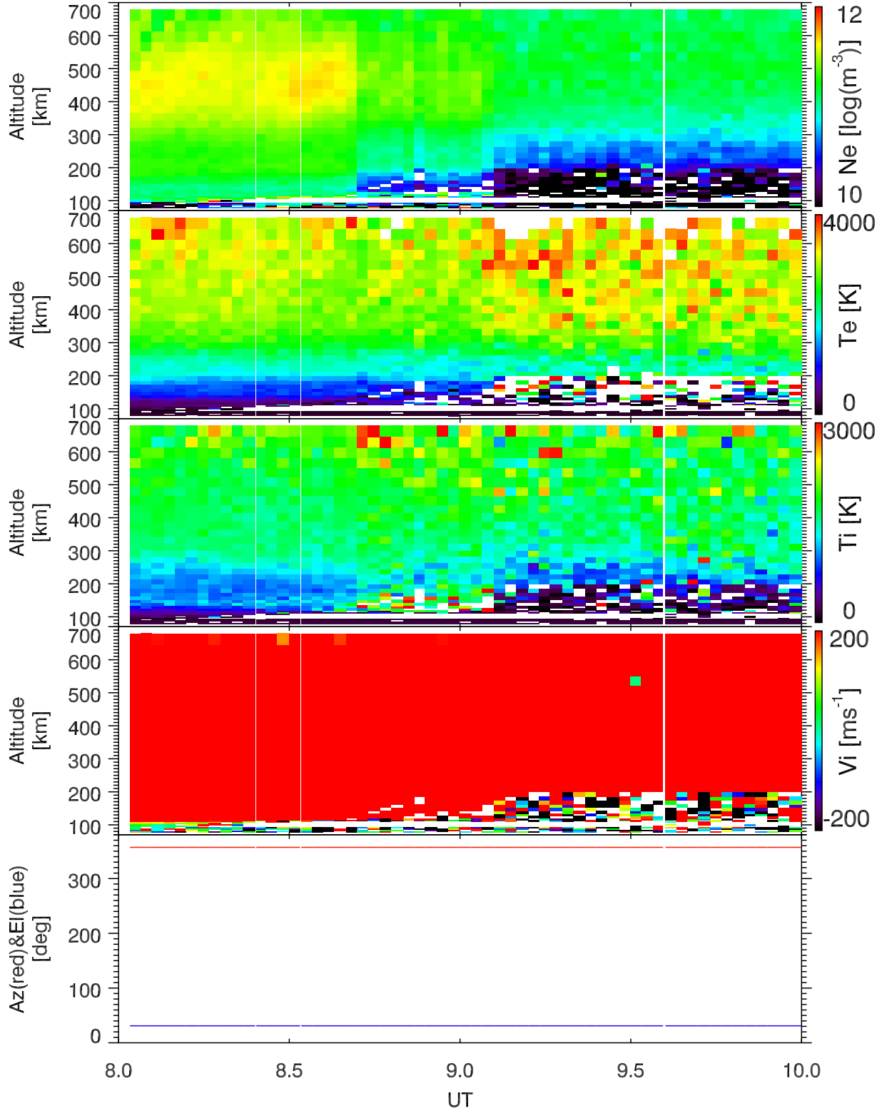
EISCAT 2000-07-20_08_10UT_tau0_120@32m.
