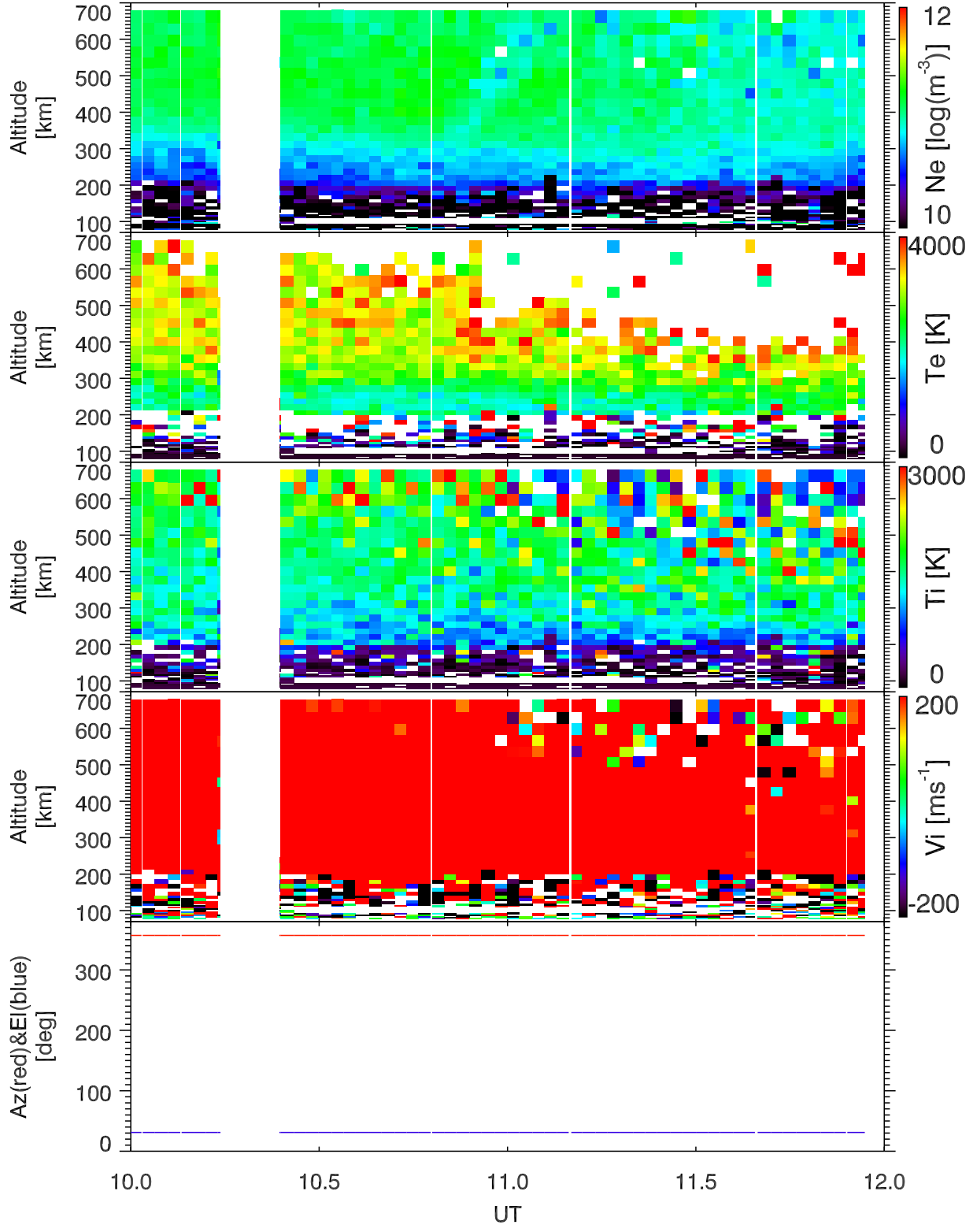
EISCAT 2000-07-20_10_12UT_tau0_120@32m.
