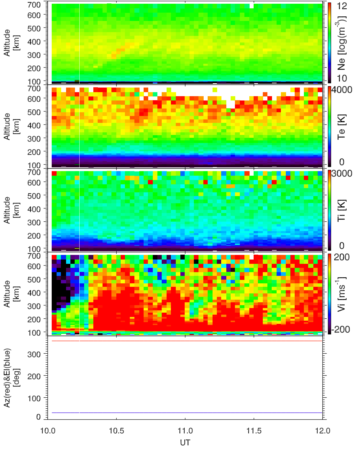
EISCAT 2000-07-21_10_12UT_tau0_120@32m.
