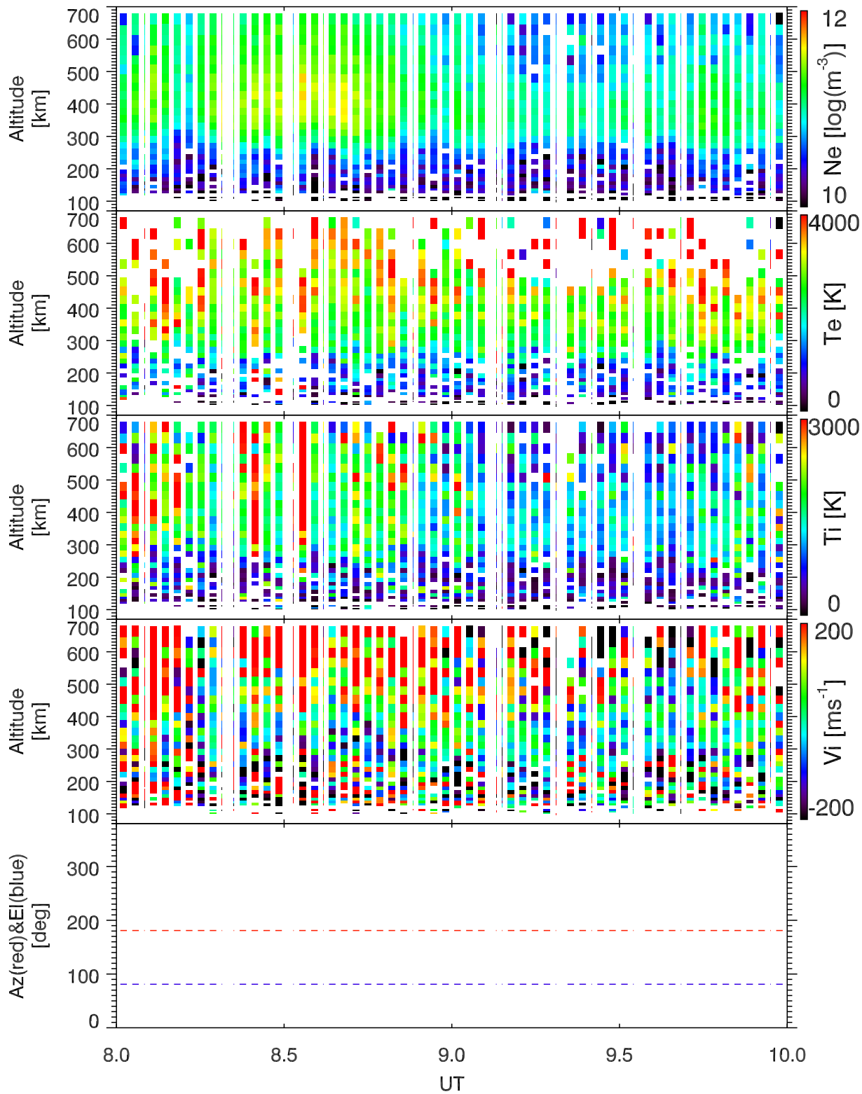
EISCAT 2001-01-21_08_10UT_tau0_all@42m.
