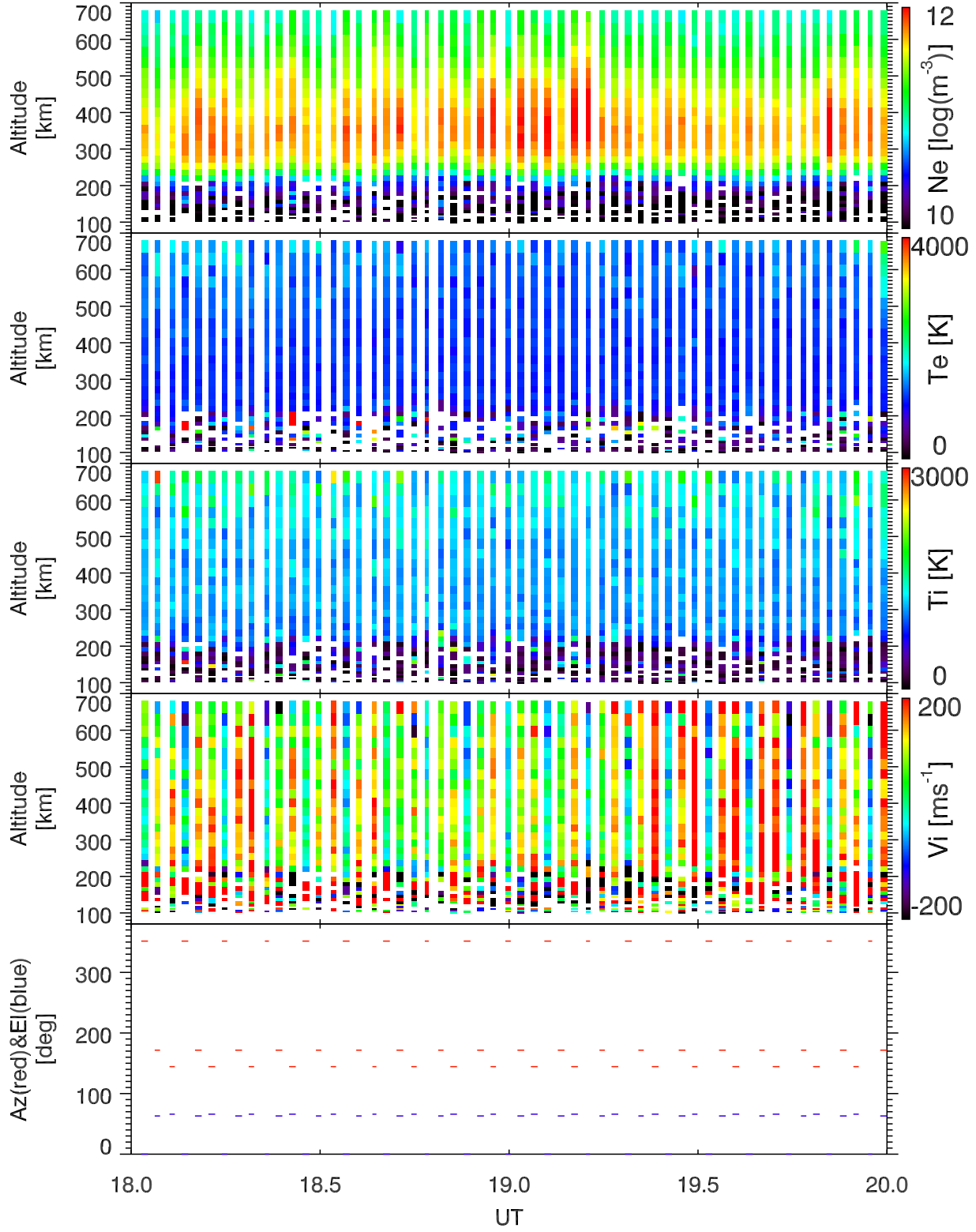
EISCAT 2001-02-19_18_20UT_tau0_ant@32m.
