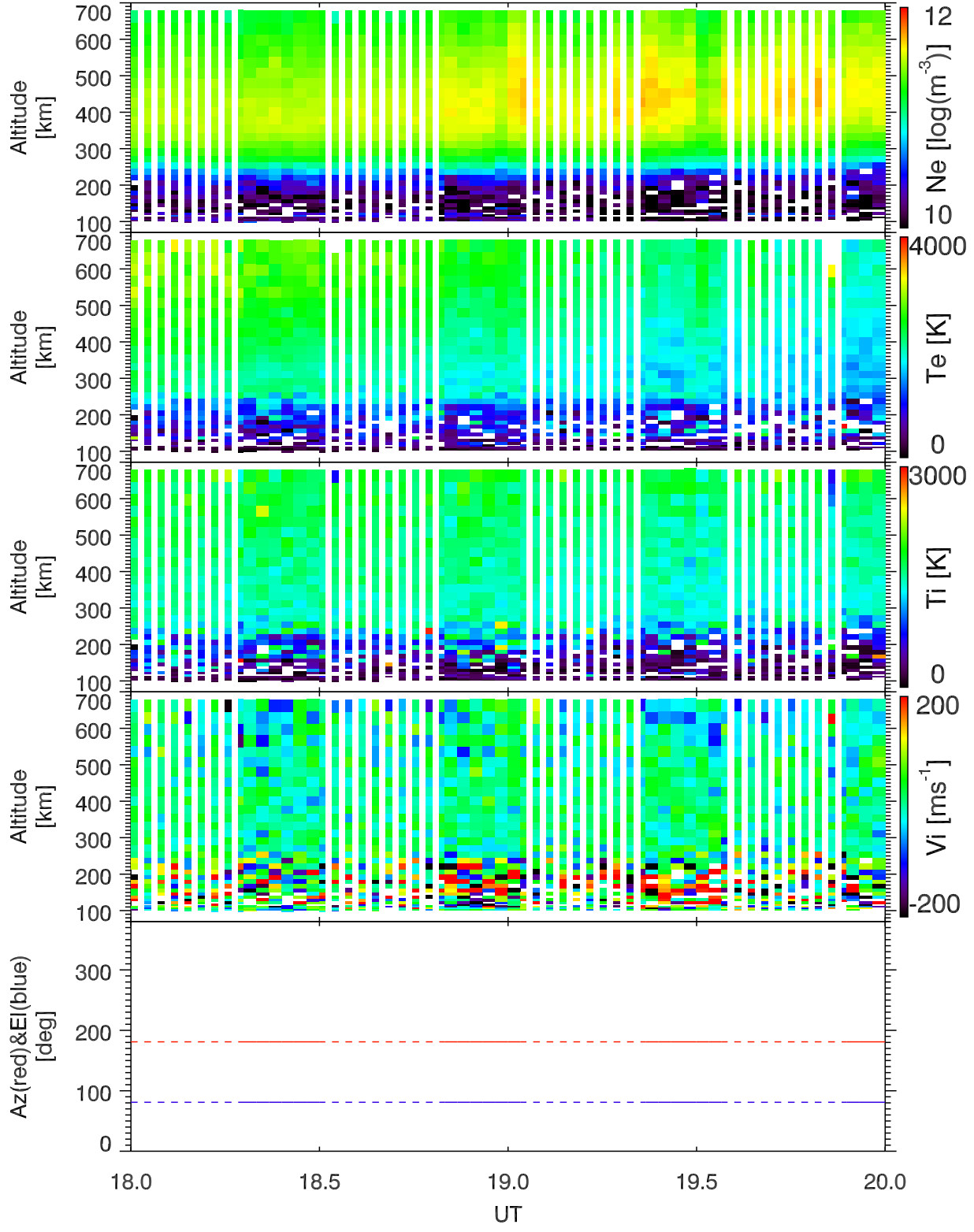
EISCAT 2001-10-01_18_20UT_tau0_120@42m.
