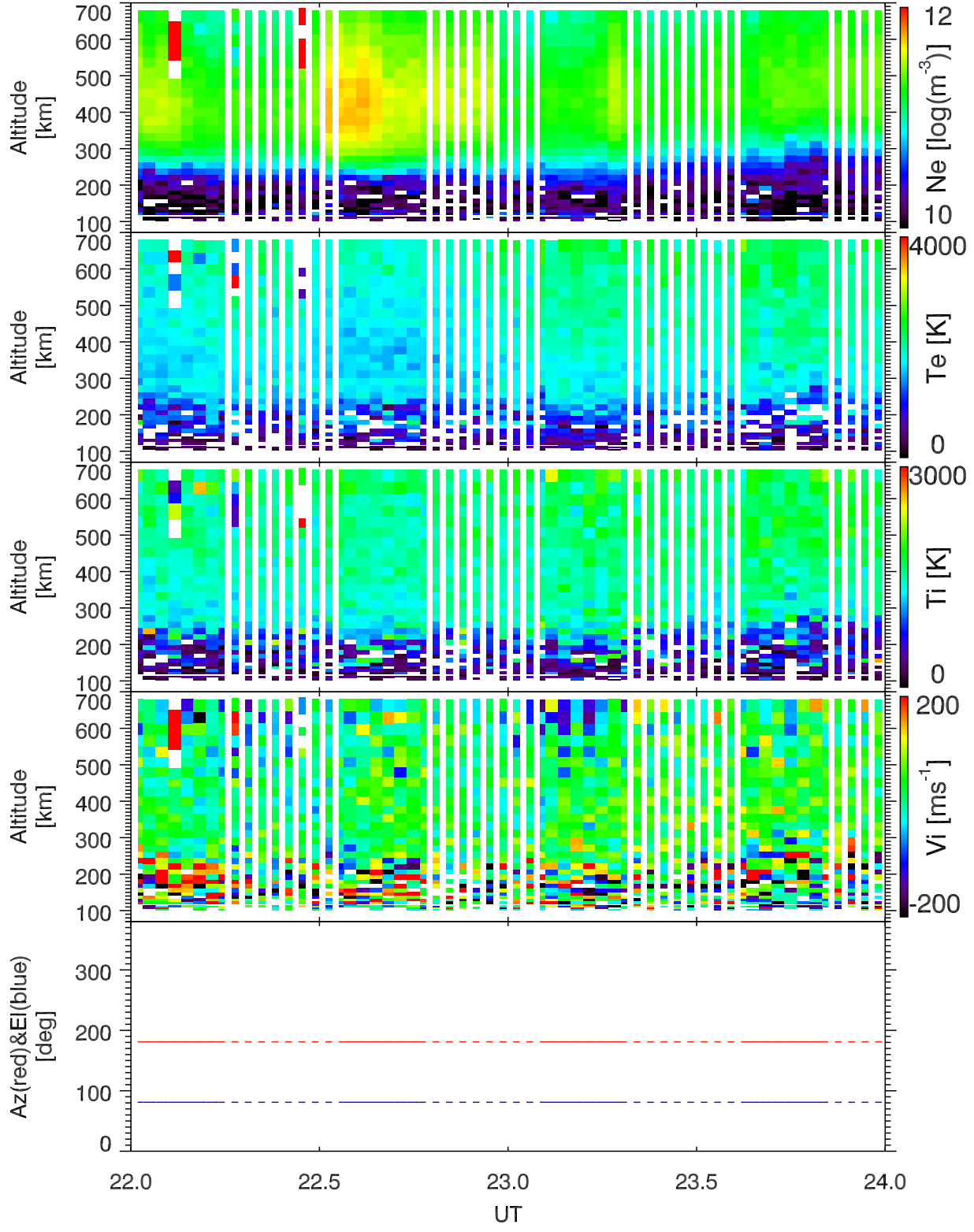
EISCAT 2001-10-01_22_24UT_tau0_120@42m.
