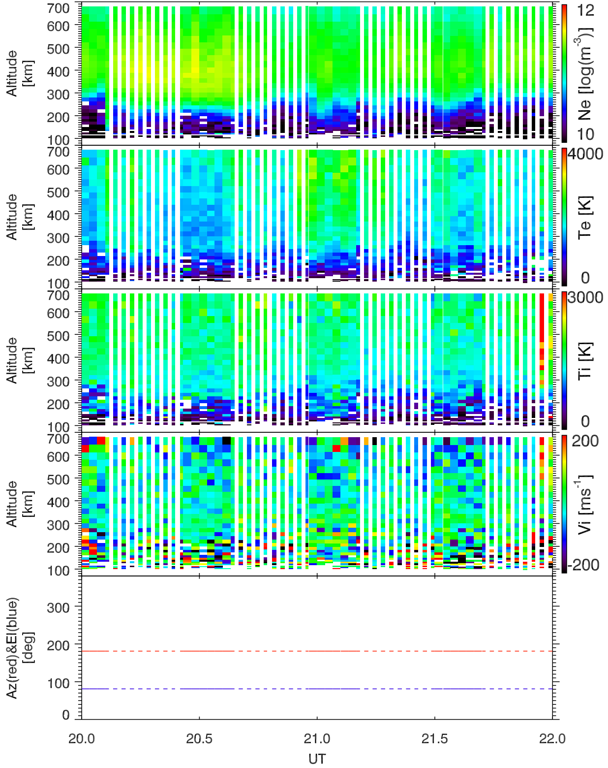
EISCAT 2001-10-09_20_22UT_tau0_120@42m.
