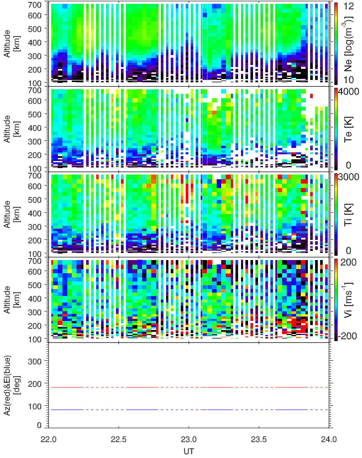
EISCAT 2001-10-09_22_24UT_tau0_120@42m.
