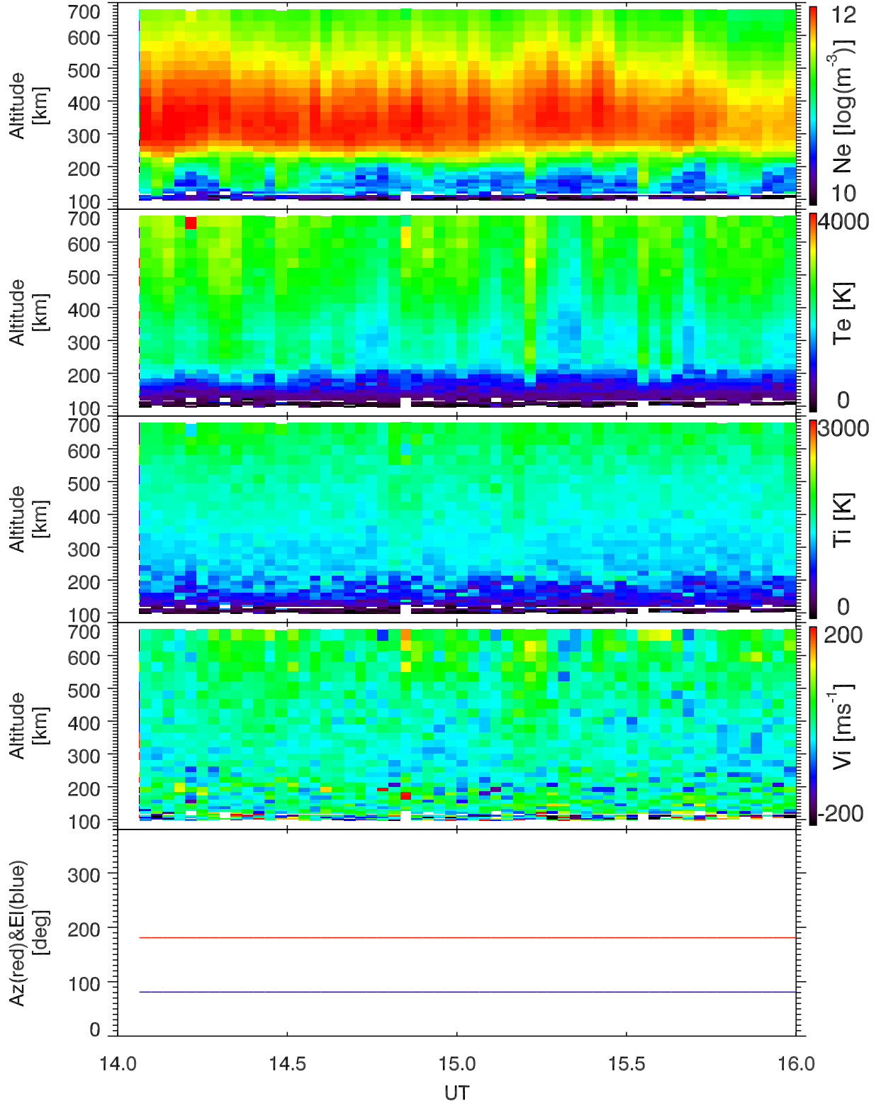
EISCAT 2001-10-16_14_16UT_tau0_120@42m.
